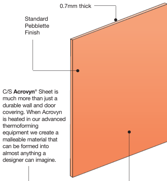
Standard Sheet 2550 x 1350mm
